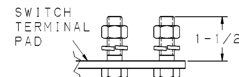
OPTION "C" CAPTIVE HARDWARE CONSIST OF 4 EACH: 1/2" STAINLESS STEEL BOLTS, LOCKWASHERS, & NUTS
